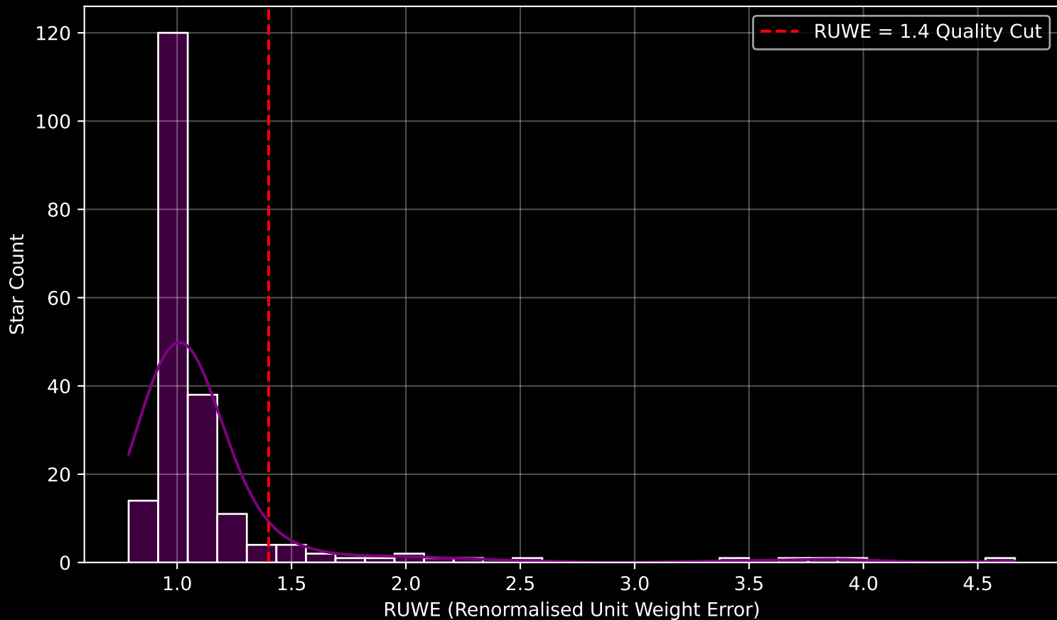
GAPOGEE DR17 Field [K2_C6_314+55] RUWE Distribution (n= 205)
