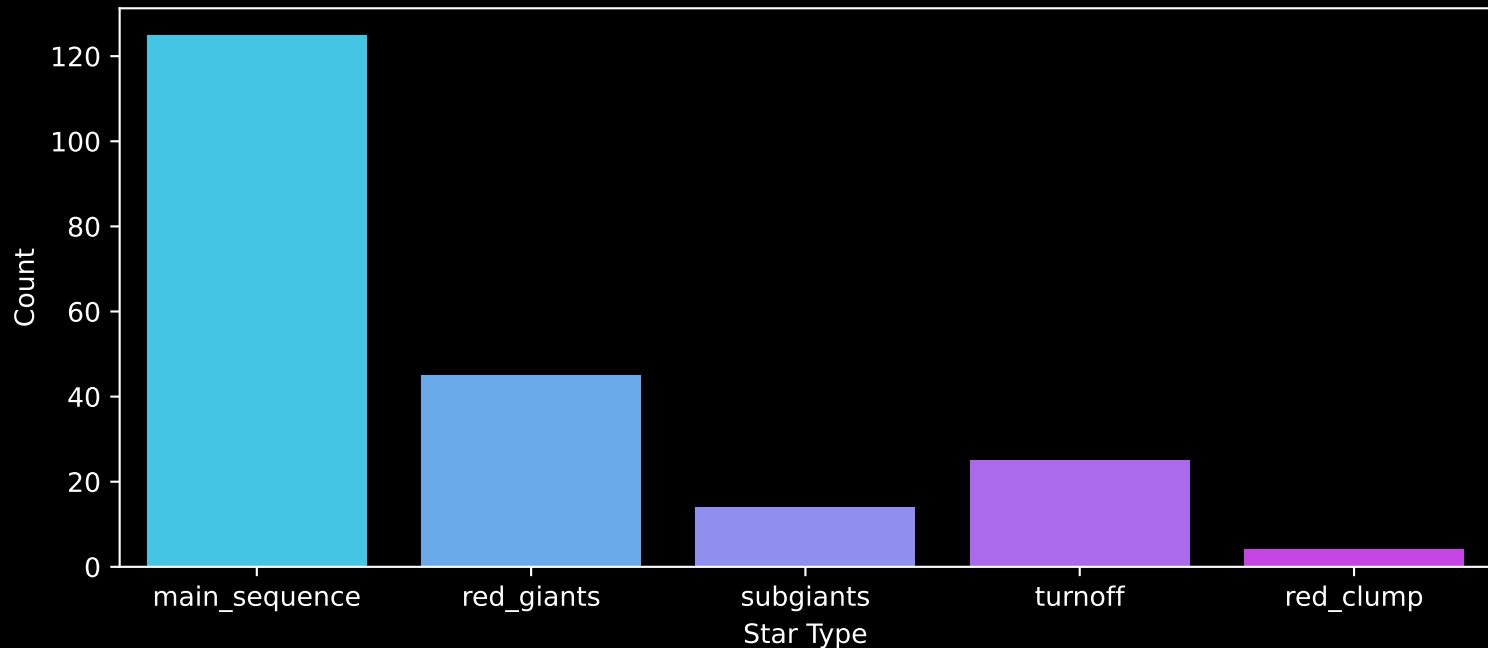
APOGEE DR17 Field: [K2_C6_314+55] Count plot of Star Type
