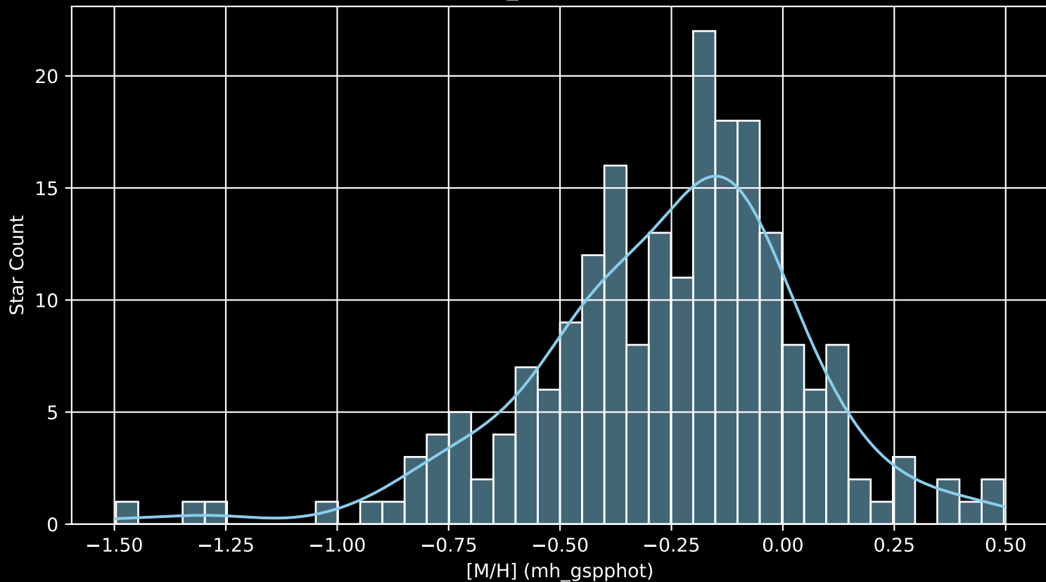
APOGEE DR17 Field: [K2_C6_314+55 [M/H] (mh_gspphot) (n= 210)
