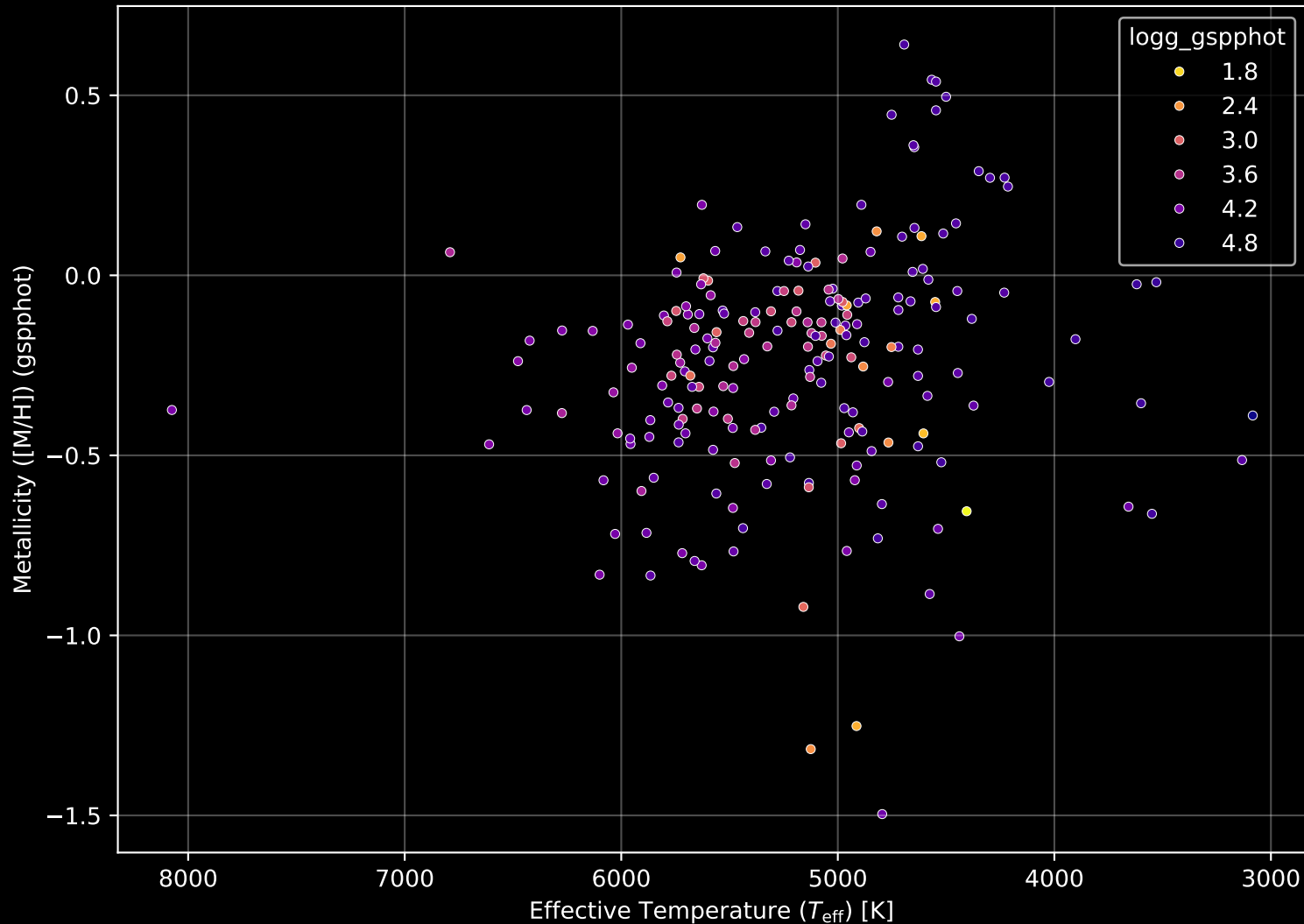
APOGEE DR17 Field: [K2_C6_314+55] Stellar Population Parameters (n= 213)
