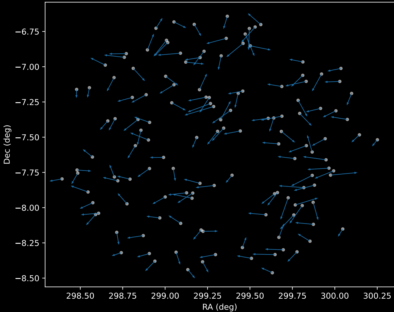
APOGEE DR17 Cluster 0 Proper Motion Vectors (n=135)
