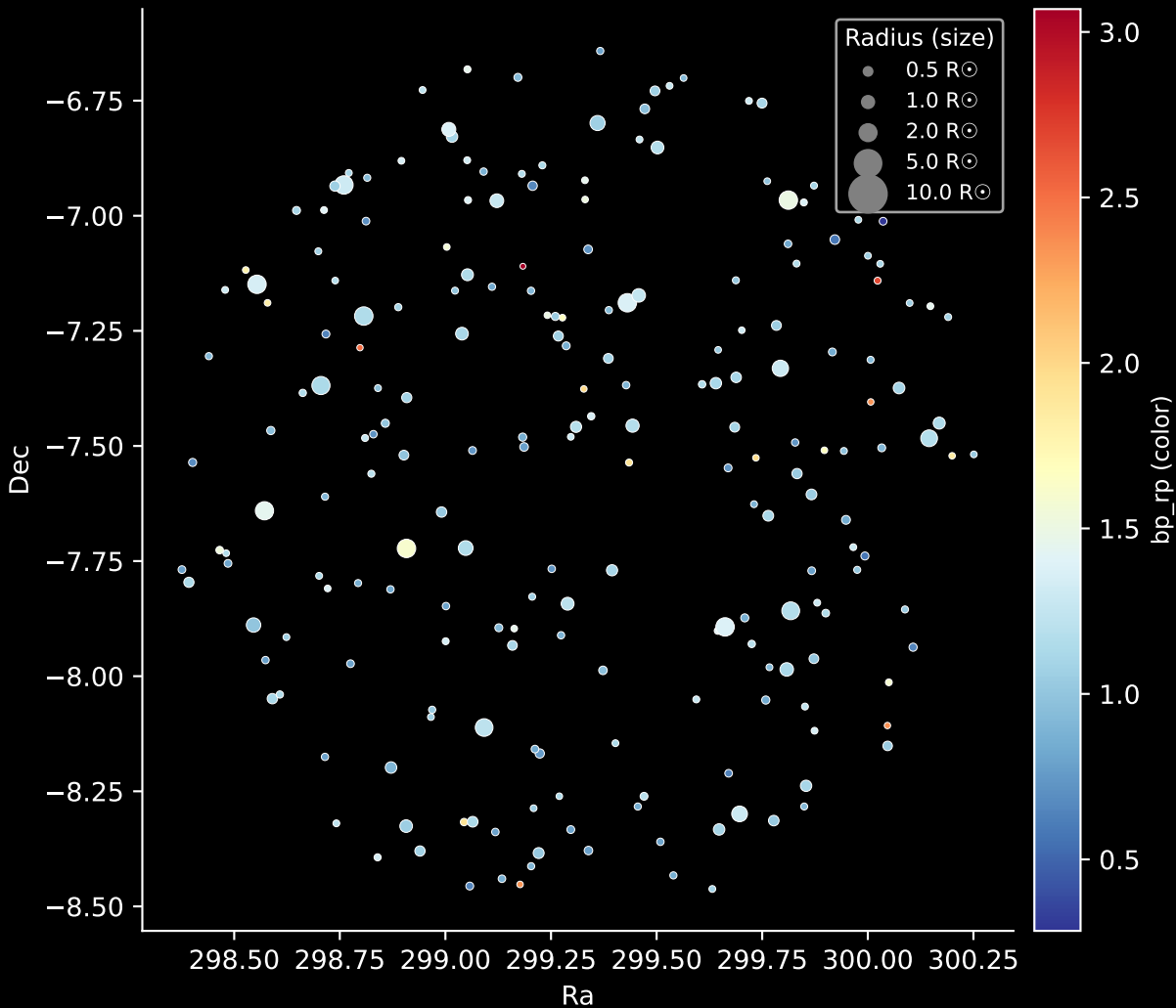
APOGEE DR17 Field: [K2_C6_314+55] Stars: 213
