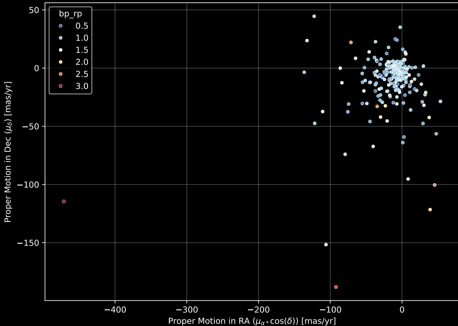
APOGEE DR17 Field: [K2_C6_314+55] Proper Motion Diagram (n= 213)
