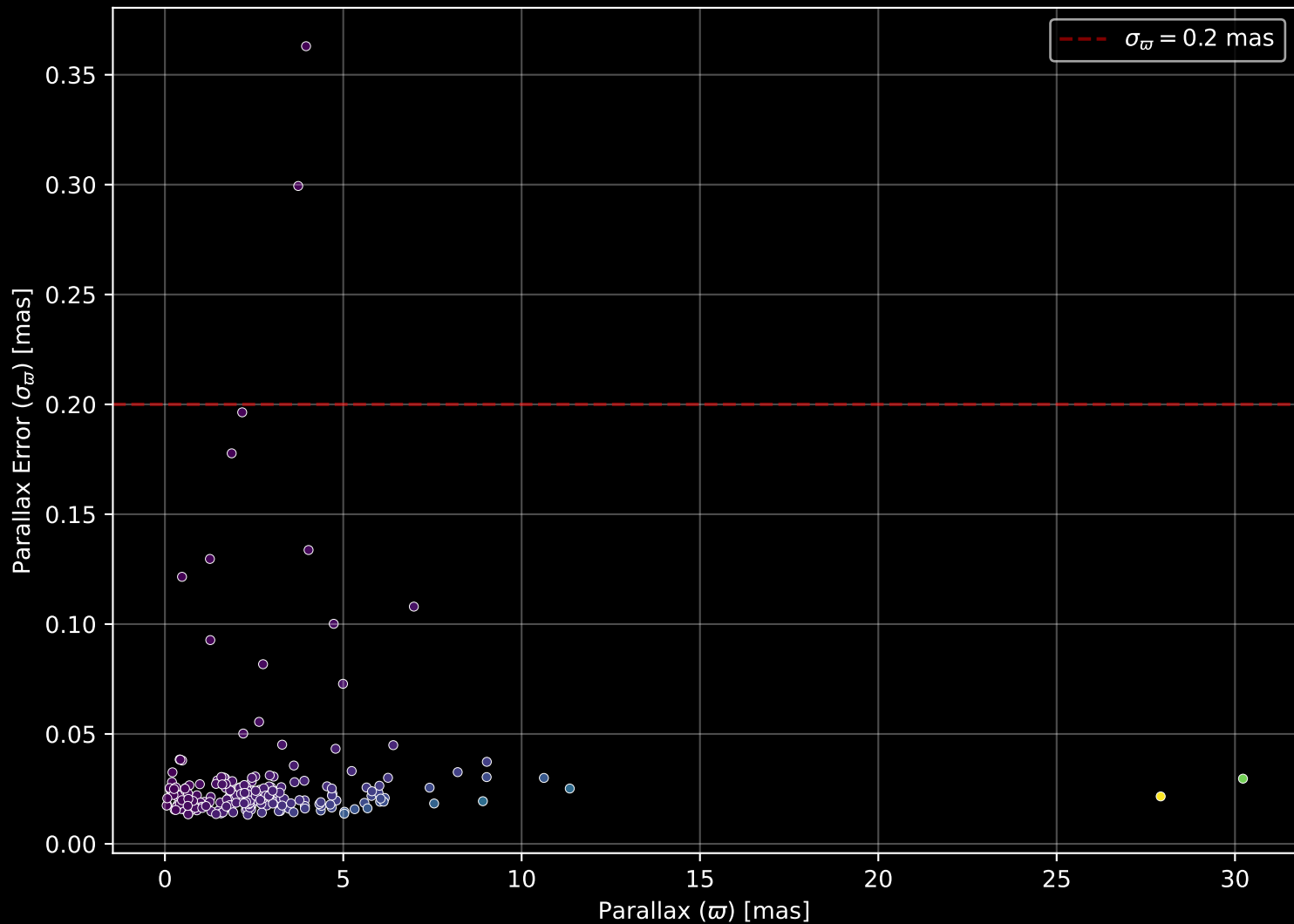
APOGEE DR17 Field: [K2_C6_314+55] Parallax Quality (n= 213)
